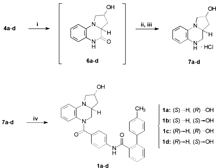
Scheme 2. i) 10% Pd-C, Et 3 N, THF, 45 °C, 4 h; ii) NaBH 4 , THF, ref., 18 h; iii) HCl; iv) 4-(4'-methyl-2-biphenylcarboxamido)benzoyl chloride, pyridine, CH 2 Cl 2 , rt, 18 h.
