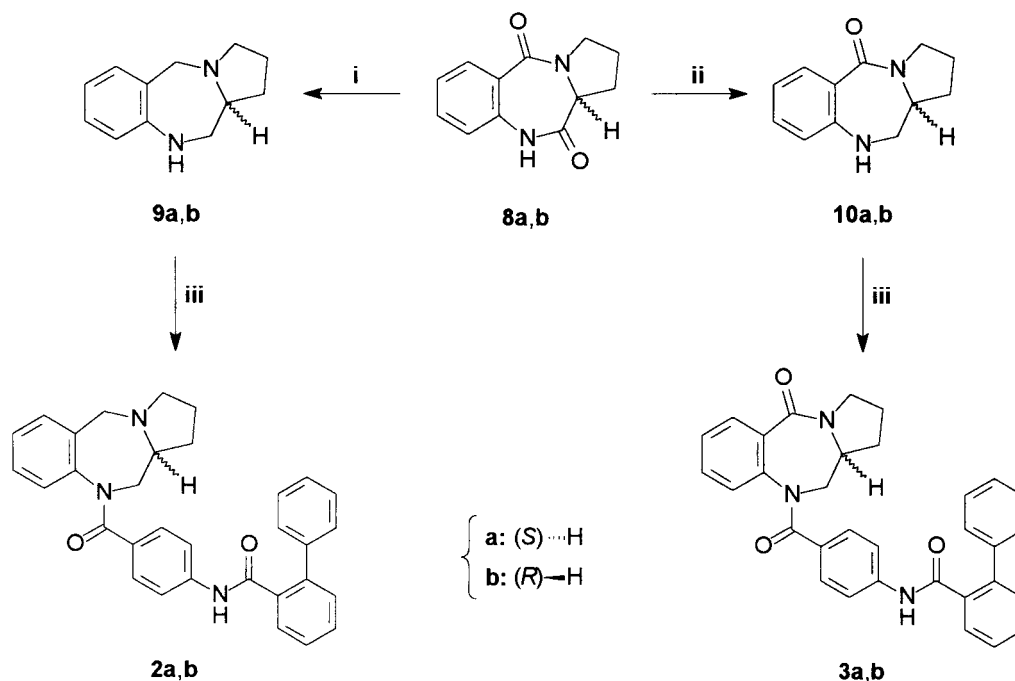
Scheme 3. i) \text{LiAlH}_4 , THF, ref., 3 h; ii) \text{NaBH}_4 , TFA, glyme, ref., 4 h; iii) 4-[(2-phenylbenzoyl)amino]benzoyl chloride, pyridine, \text{CH}_2\text{Cl}_2 , rt, 18 h
