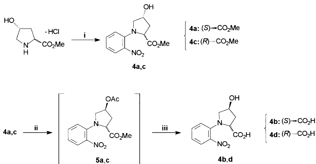
Scheme 1. i) 1-fluoro-2-nitrobenzene, Et 3 N, CH 3 CN, 60 °C, 16 h; ii) Ph 3 P, DIPAD, AcOH, toluene, rt, 2 h; iii) 1. aq. NaOH, rt, 20 h 2.HCl
